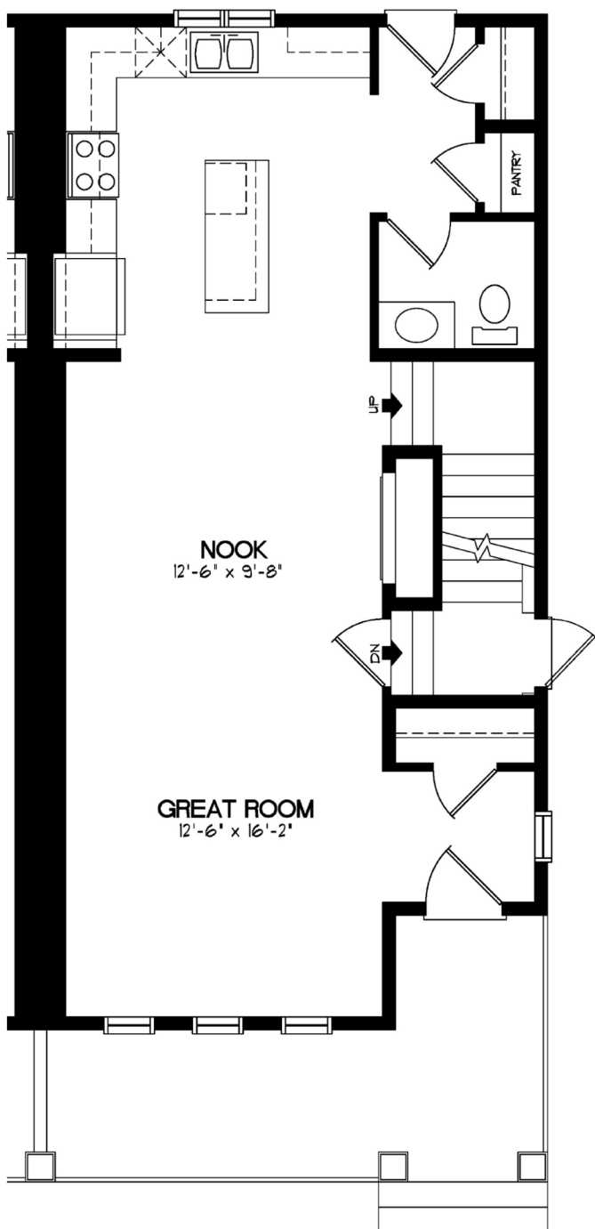
MAIN FLOOR - 773 SQFT
