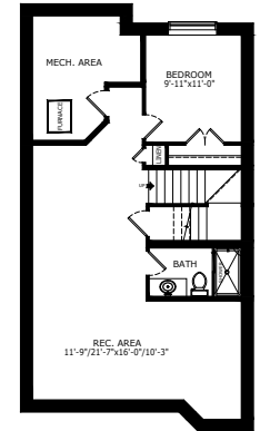
1 BEDROOM 'LEGAL SUITE' 719 SQ FT
