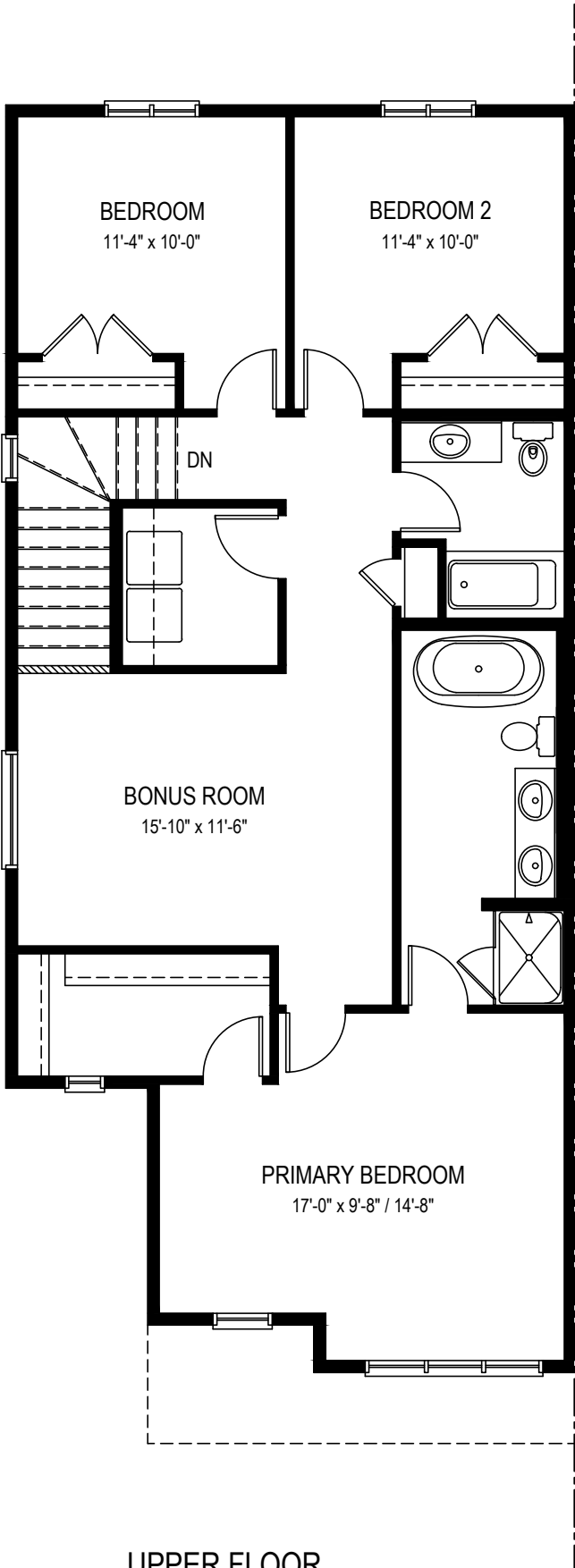
UPPER FLOOR 1198 sq.ft.
