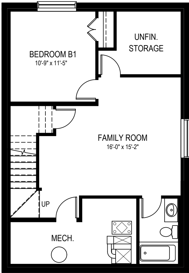
BASEMENT DEVELOPMENT OPTION 489 sq.ft.
