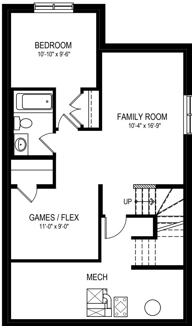
BASEMENT DEVELOPMENT OPTION 543 sq.ft.
