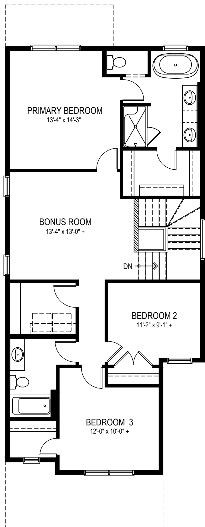
UPPER FLOOR 1152 sq.ft.
