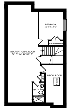
1 BEDROOM 'LEGAL SUITE' 818 SQ FT
